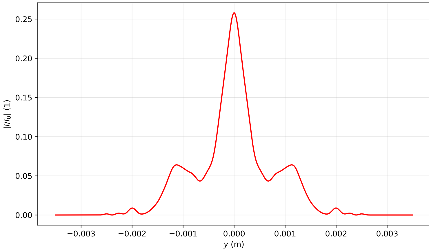
Intensity profile I(x = 0, y, z = 2.866)/I_0 , P_{in}=5.5P_{cr} , artificial time
